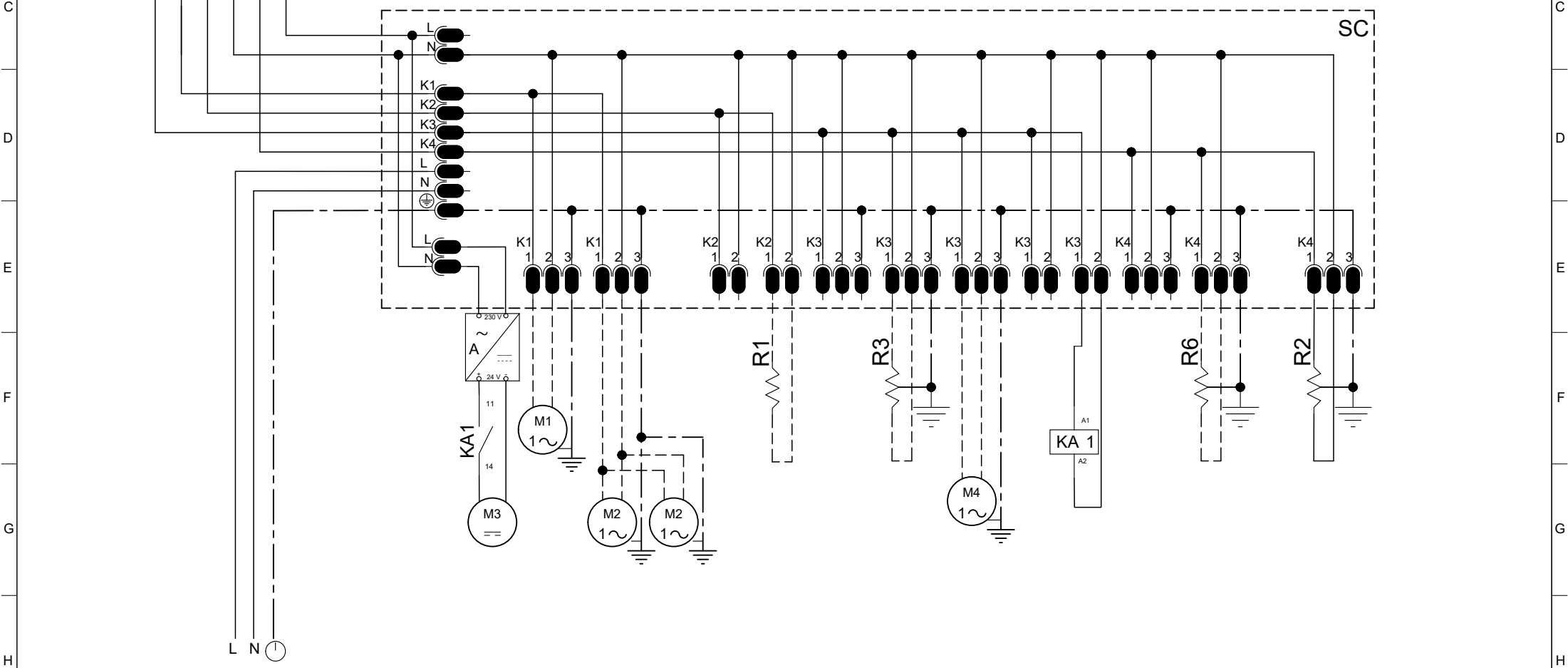
WIRING DIAGRAM POP COUNTER 230V/1/50-60Hz
