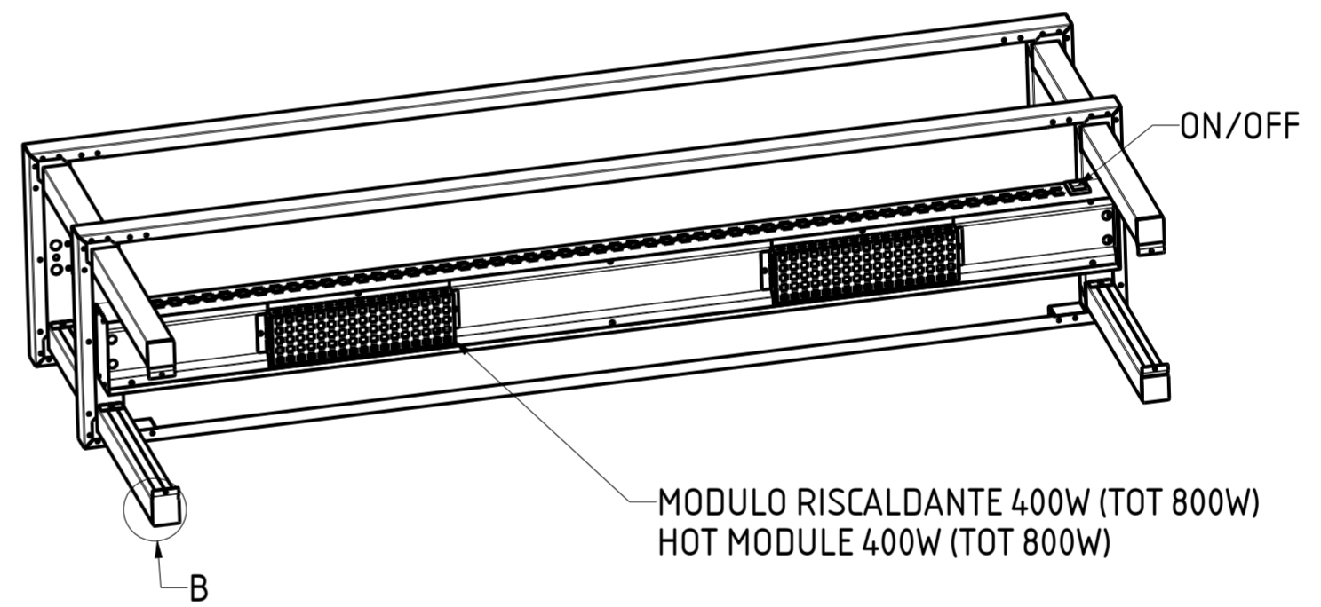
3D BOTTOM VIEW 1:10
