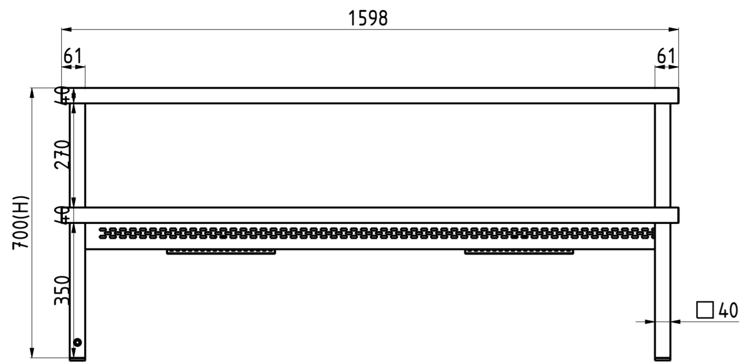
FRONT VIEW 1:10
