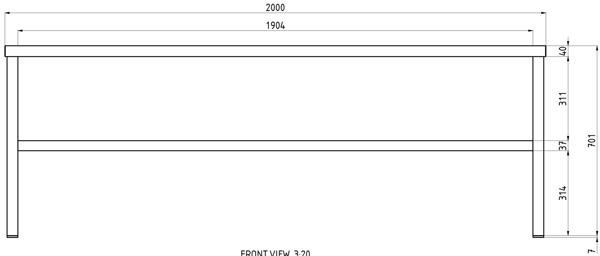
FRONT VIEW 3:20
