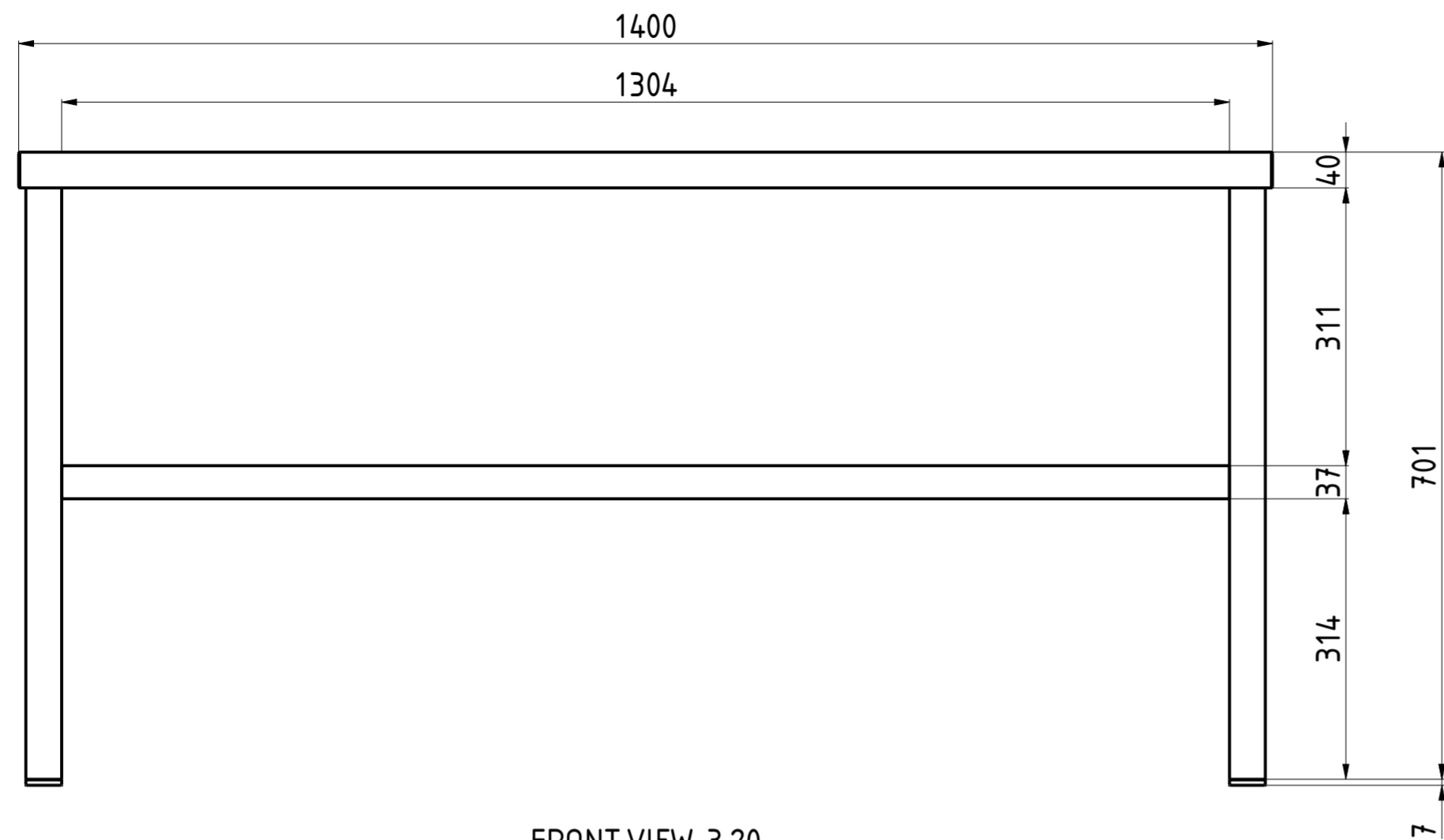
FRONT VIEW 3:20
