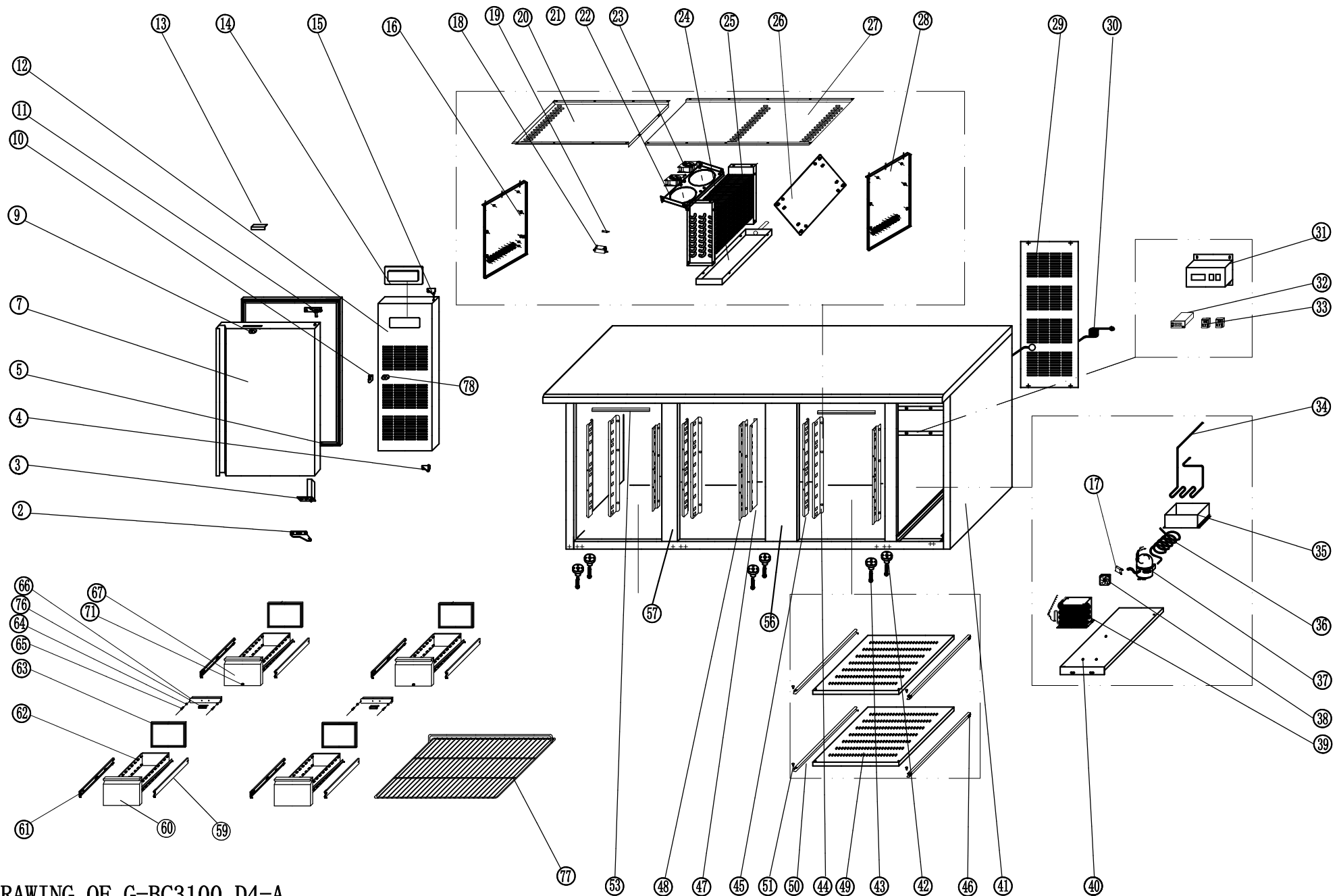
EXPLODE DRAWING OF G-BC3100 D4-A
