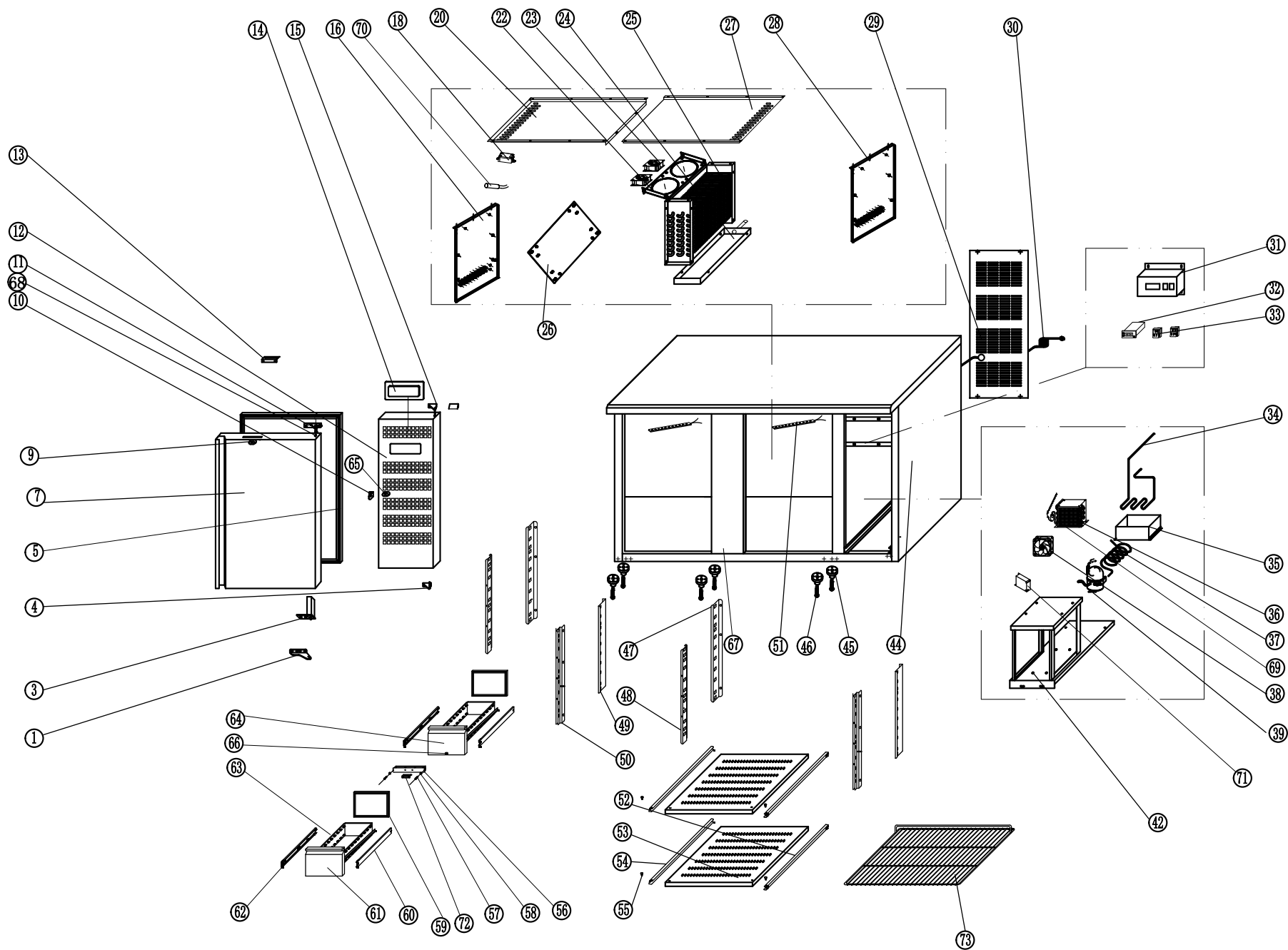
EXPLODE DRAWING OF G-BC2100 2D-A
