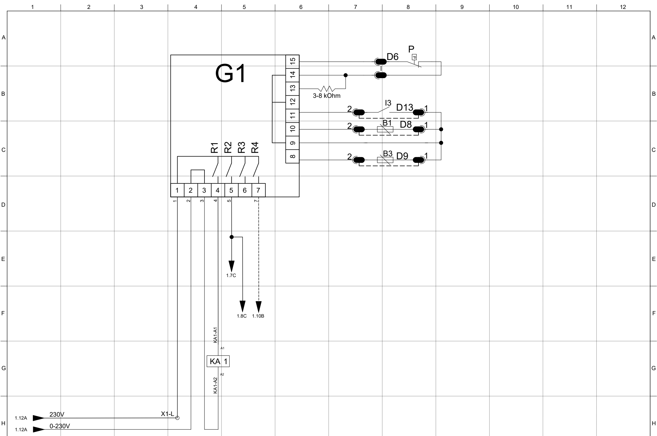
WIRING DIAGRAM COMPACT BLAST CHILLER 051-081 230/1/50-60Hz
