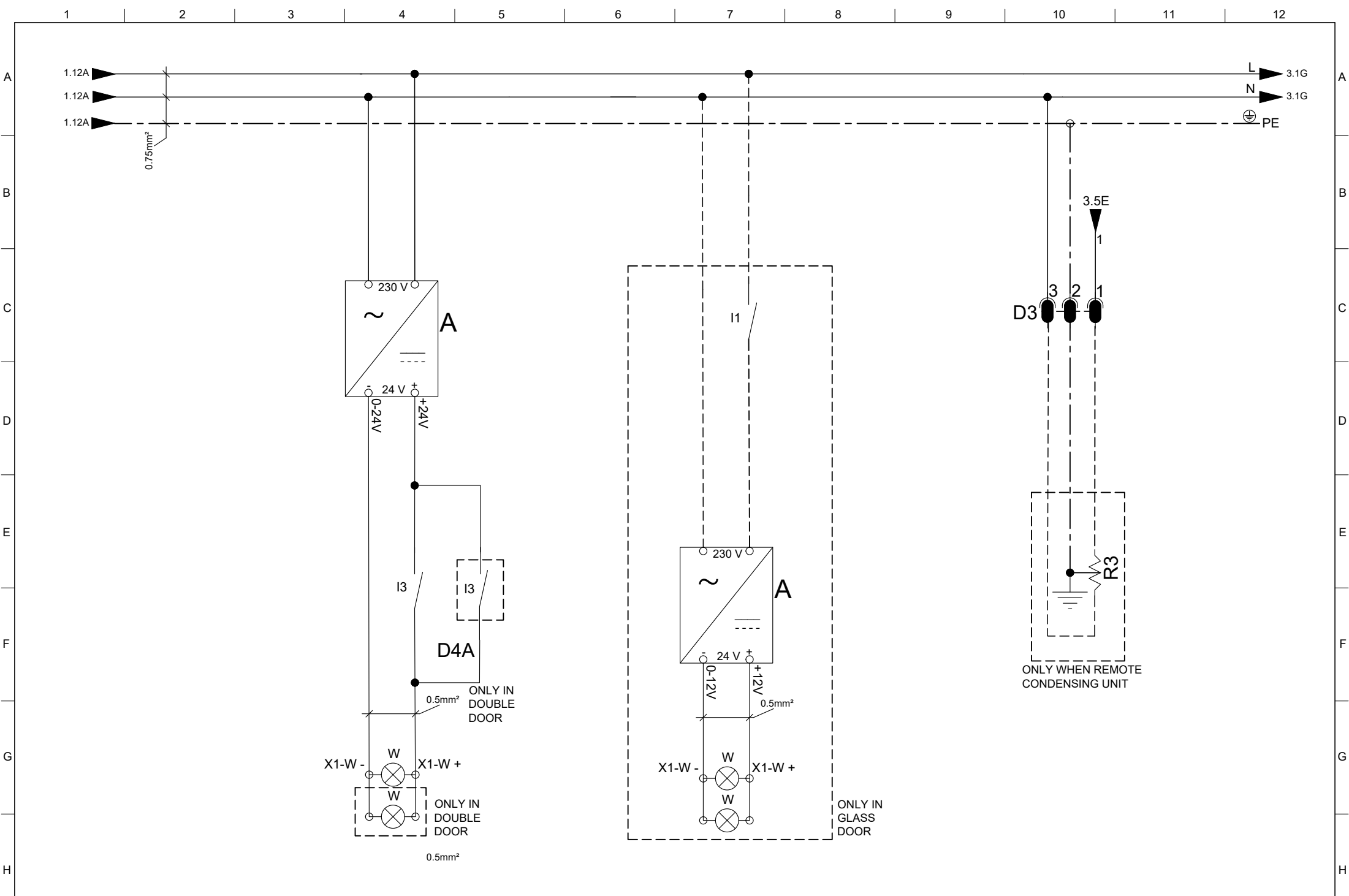
WIRING DIAGRAM CHERRY CABINET 230/1/50-60Hz
